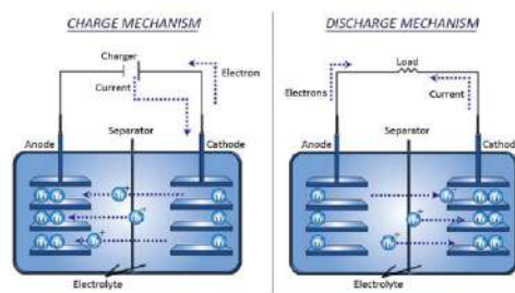
Figure 2.1 Charge and discharge mechanism of Li-ion batteries [10]
